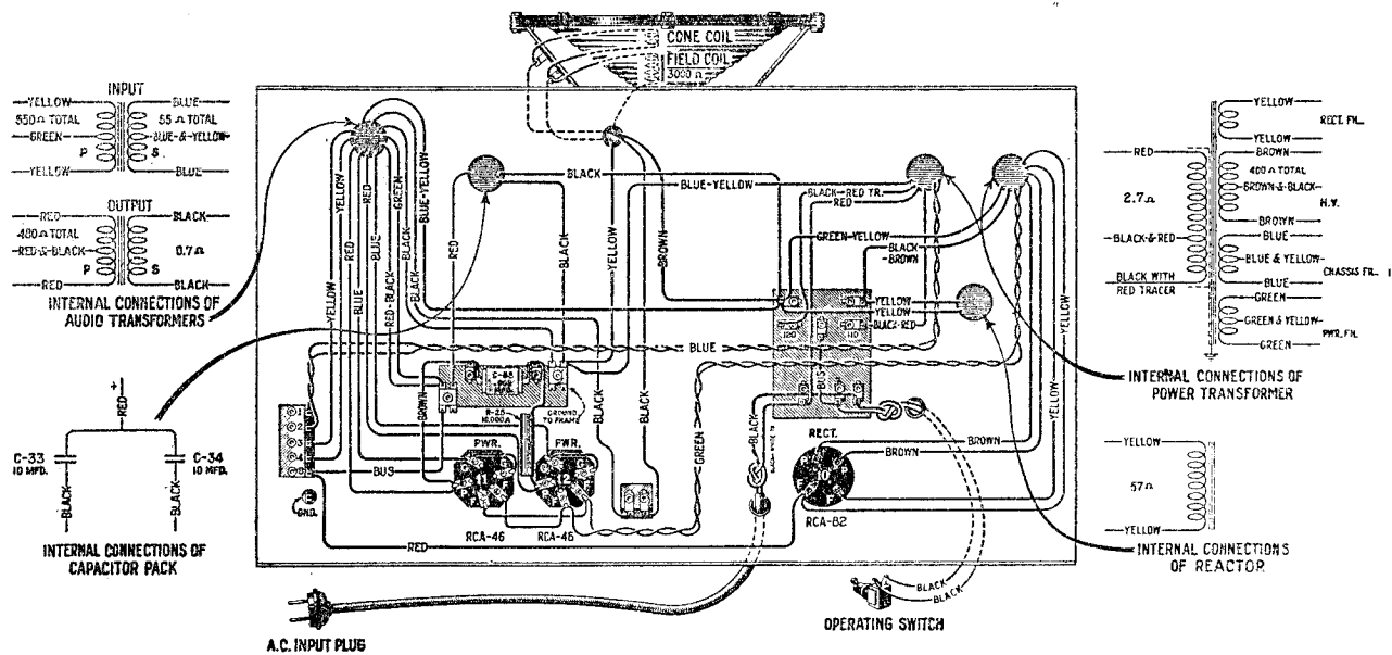
Figure 3—Amplifier Wiring Diagram of RAE 84
